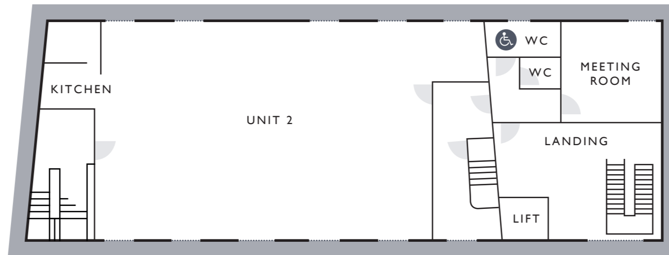
FIRST FLOOR | BATH LANE MILL
